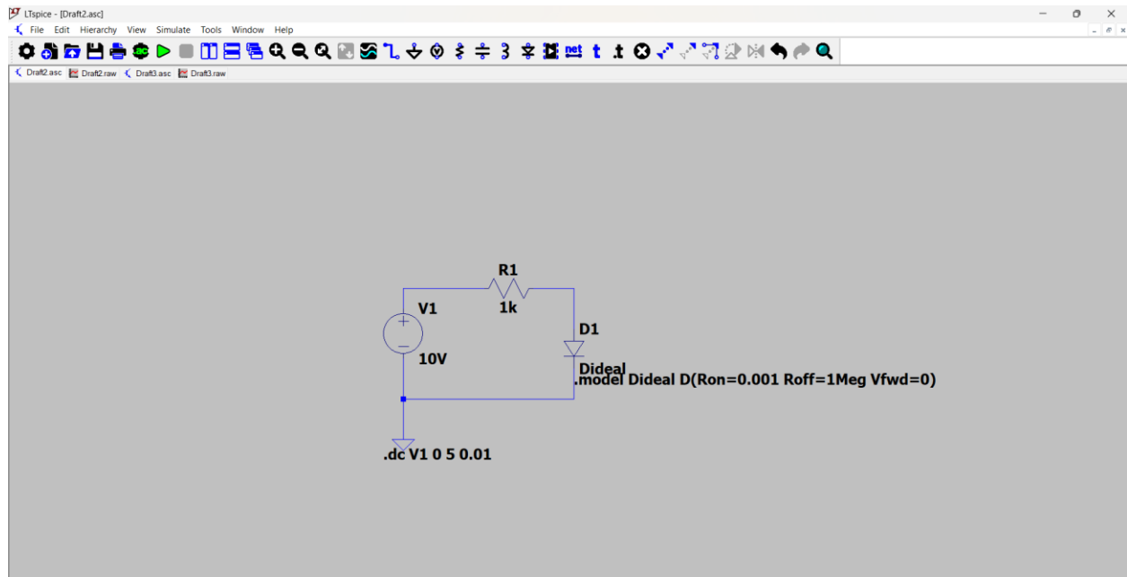
Figure 1: Ideal Diode Schematic View
